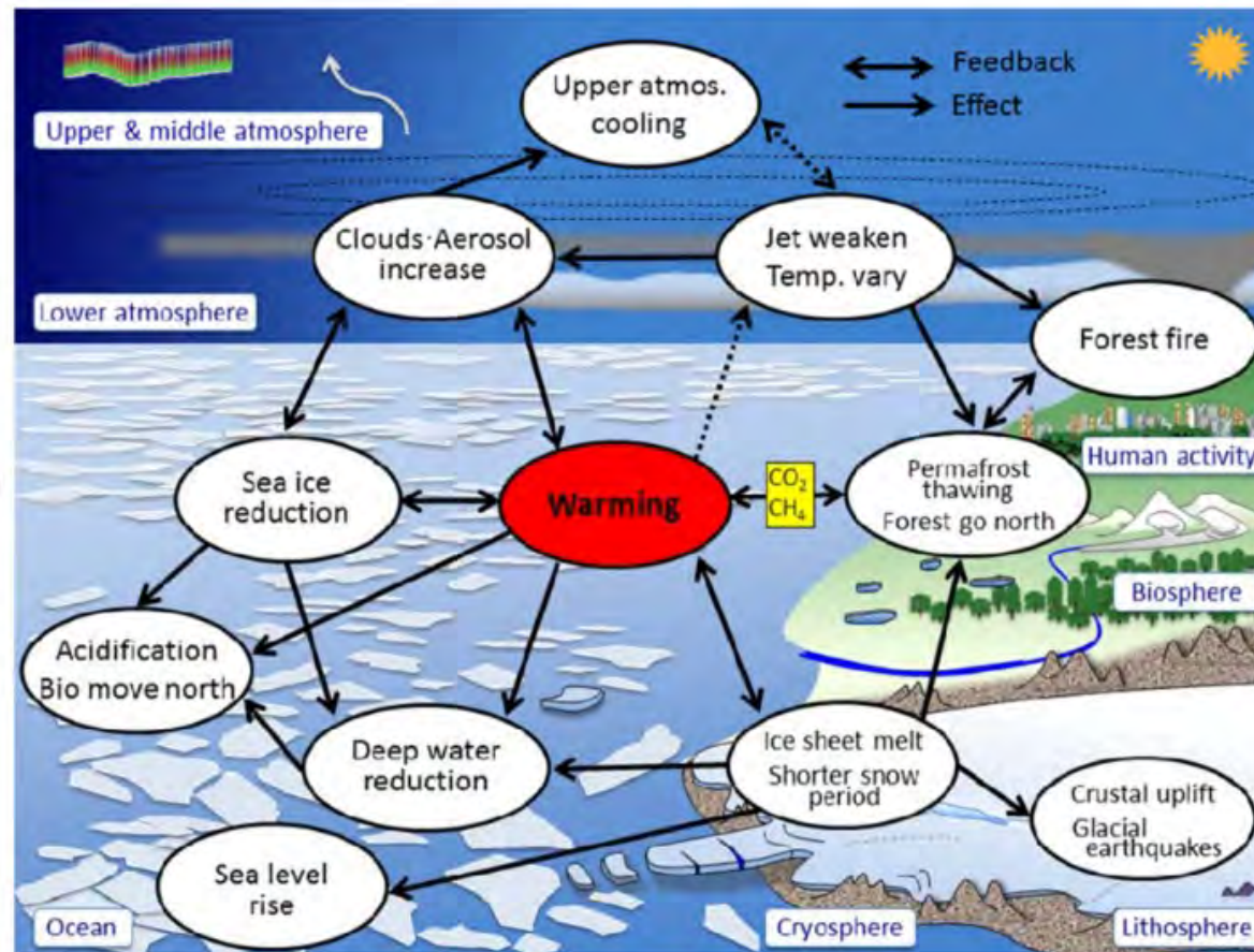
Crucial changes in the atmosphere, land, cryosphere and ocean, in response to current climate change, along with the effects (one way) and feedback (two ways). Note that while only major changes and interactions are displayed, other variations may exist. The solid arrows denote confirmed interactions, and the dotted ones denote more hypothetical ones. Also, the interactions between clouds and global warming can work both ways: e.g., the presented feedback is important in seasons other than summer, although clouds shield solar radiation and reduce sea ice melting in summer. In addition, forest fires occur without global warming, but are becoming more frequent.
